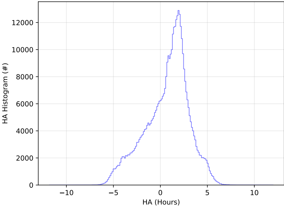
too_combined_s0.5_v3.4_10yrs All sky z band: HA Histogram
