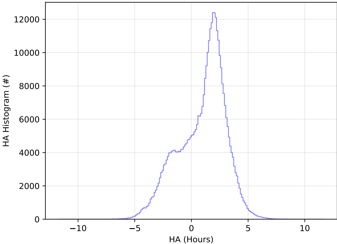
too_combined_s0.5_v3.4_10yrs All sky y band: HA Histogram
