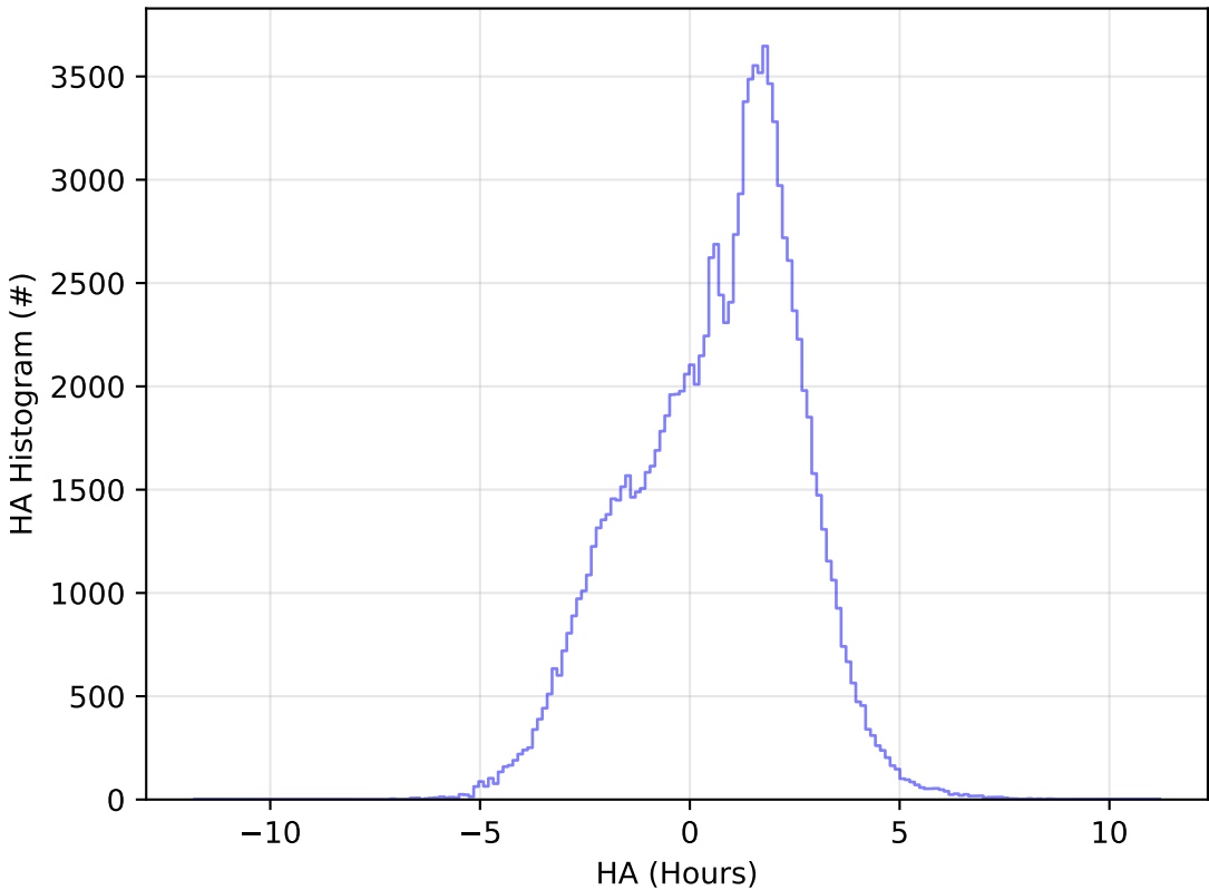
too_combined_s0.5_v3.4_10yrs All sky u band: HA Histogram
