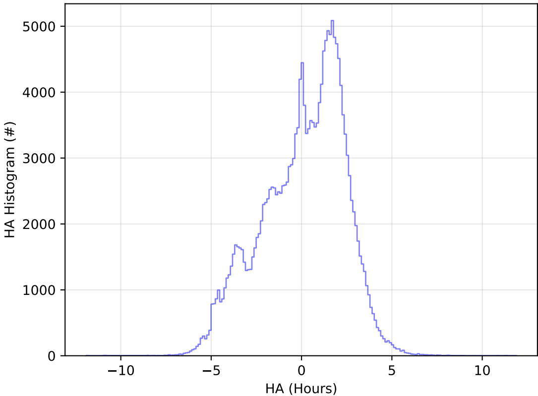
too_combined_s0.5_v3.4_10yrs All sky g band: HA Histogram
