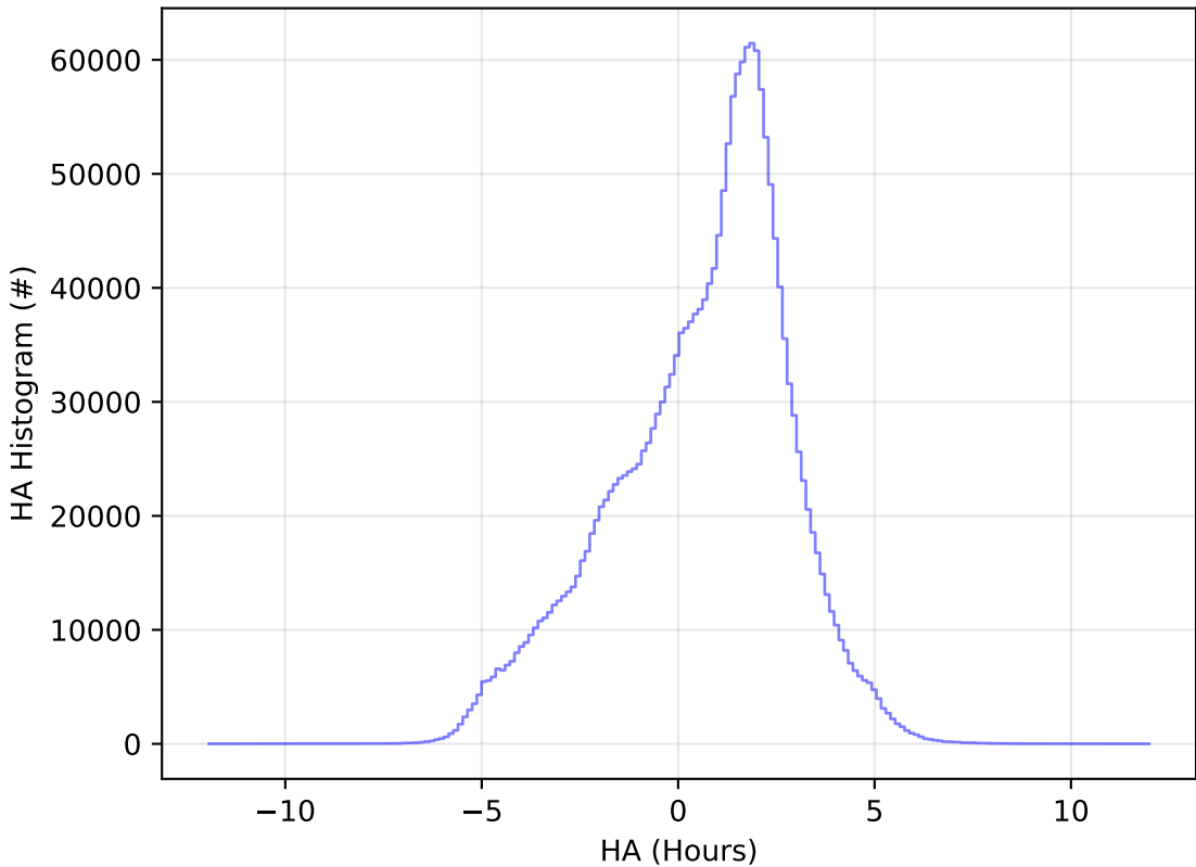
too_combined_s0.5_v3.4_10yrs All sky all bands: HA Histogram
