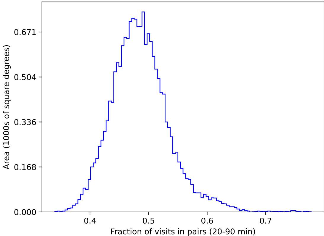
too_combined_s0.5_v3.4_10yrs gri WFD: Fraction of visits in pairs (20-90 min)
