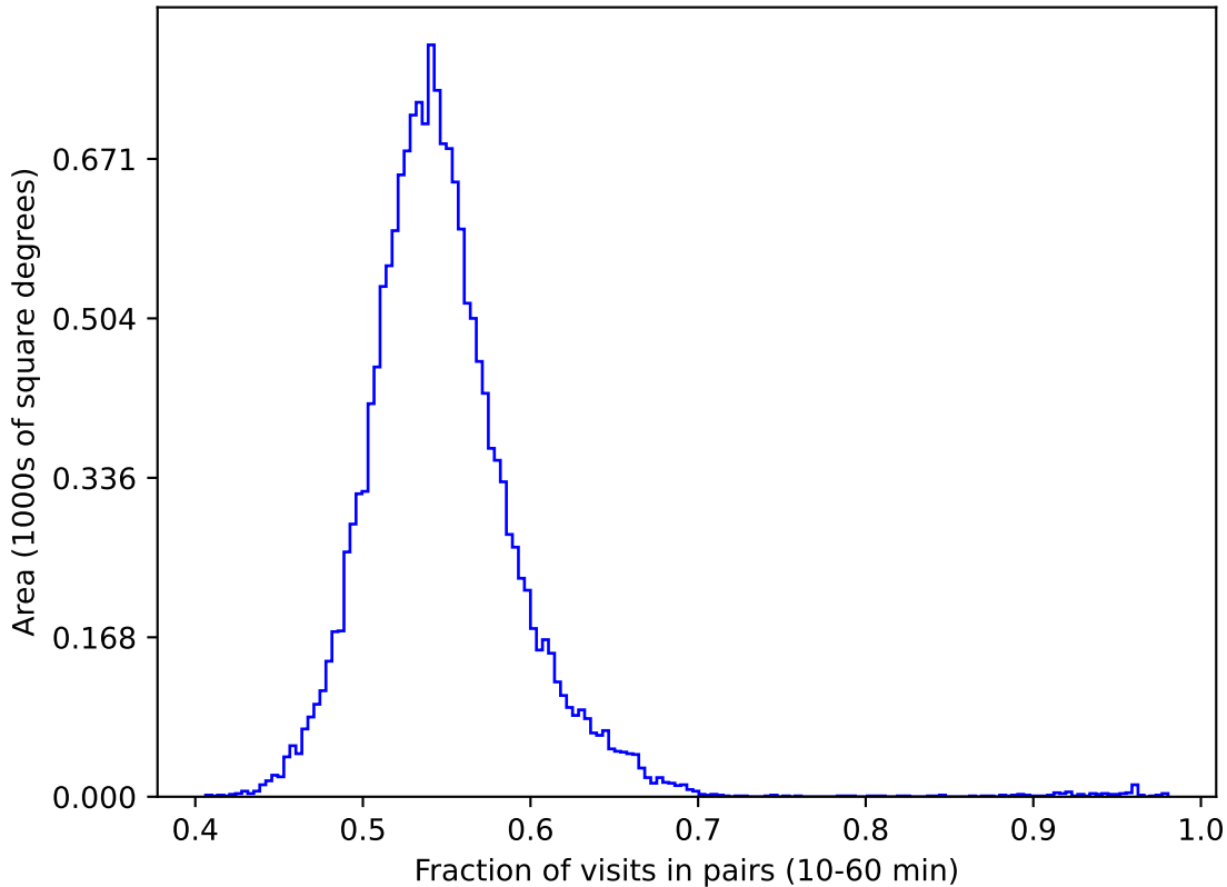
too_combined_s0.5_v3.4_10yrs gri WFD: Fraction of visits in pairs (10-60 min)
