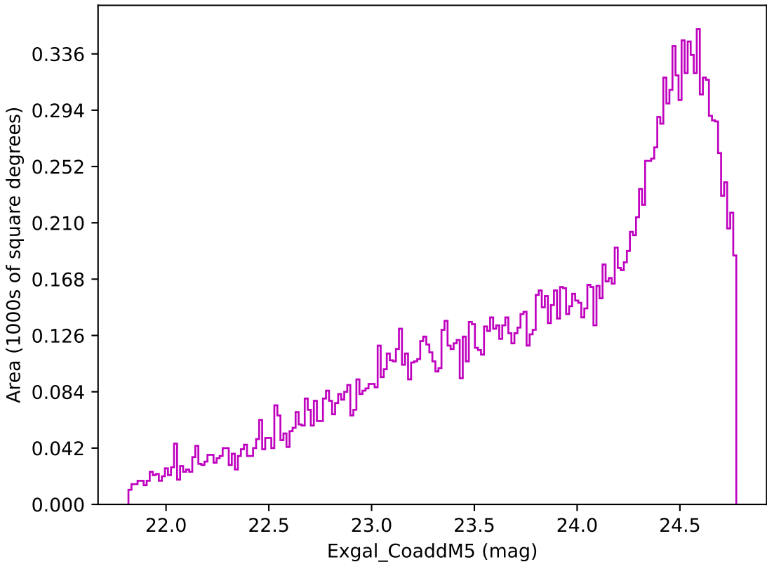
too_combined_s0.5_v3.4_10yrs Yr 3-4 z band: Exgal_CoaddM5
