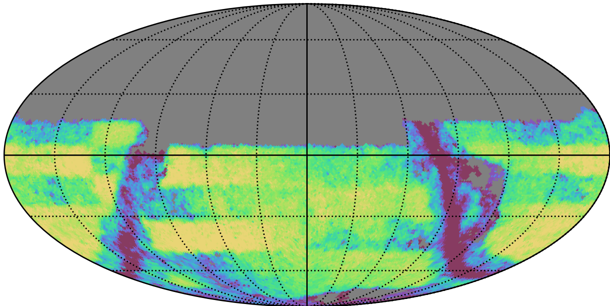
too_combined_s0.5_v3.4_10yrs Yr 3-4 y band: Exgal_CoaddM5
