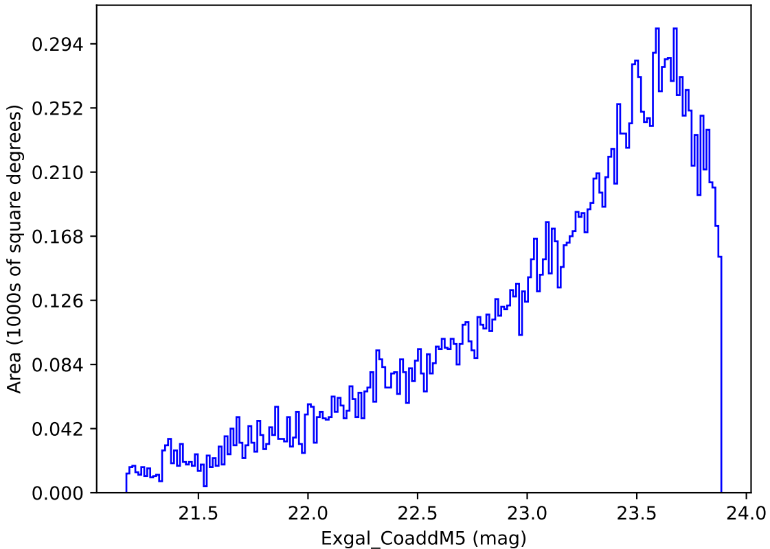
too_combined_s0.5_v3.4_10yrs Yr 3-4 y band: Exgal_CoaddM5
