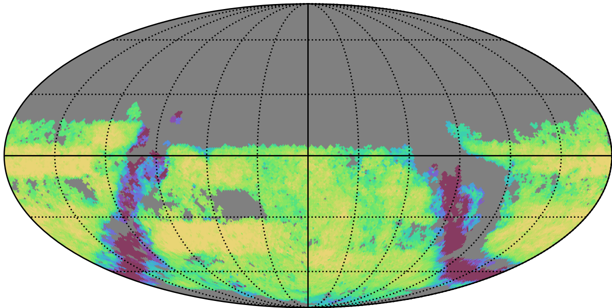
too_combined_s0.5_v3.4_10yrs Yr 3-4 u band: Exgal_CoaddM5
