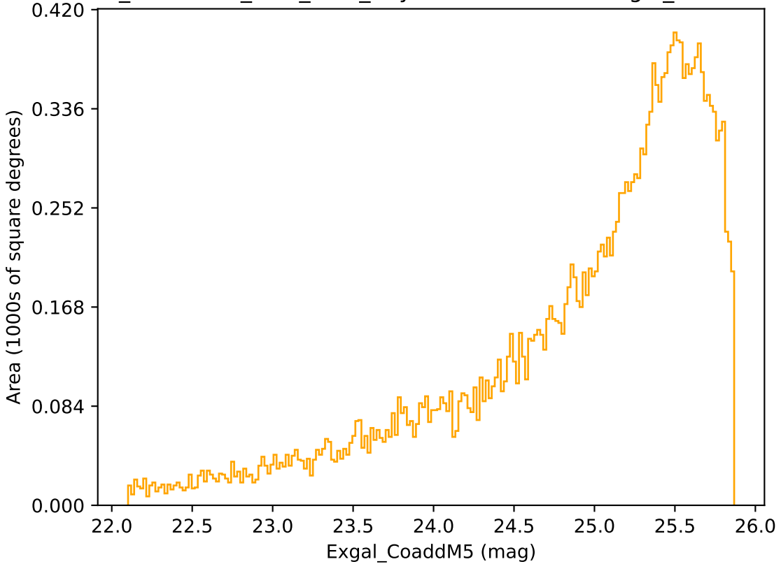
too_combined_s0.5_v3.4_10yrs Yr 3-4 r band: Exgal_CoaddM5
