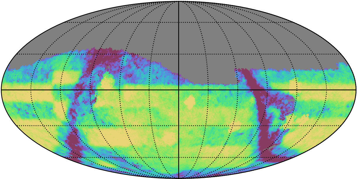
too_combined_s0.5_v3.4_10yrs Yr 3-4 i band: Exgal_CoaddM5
