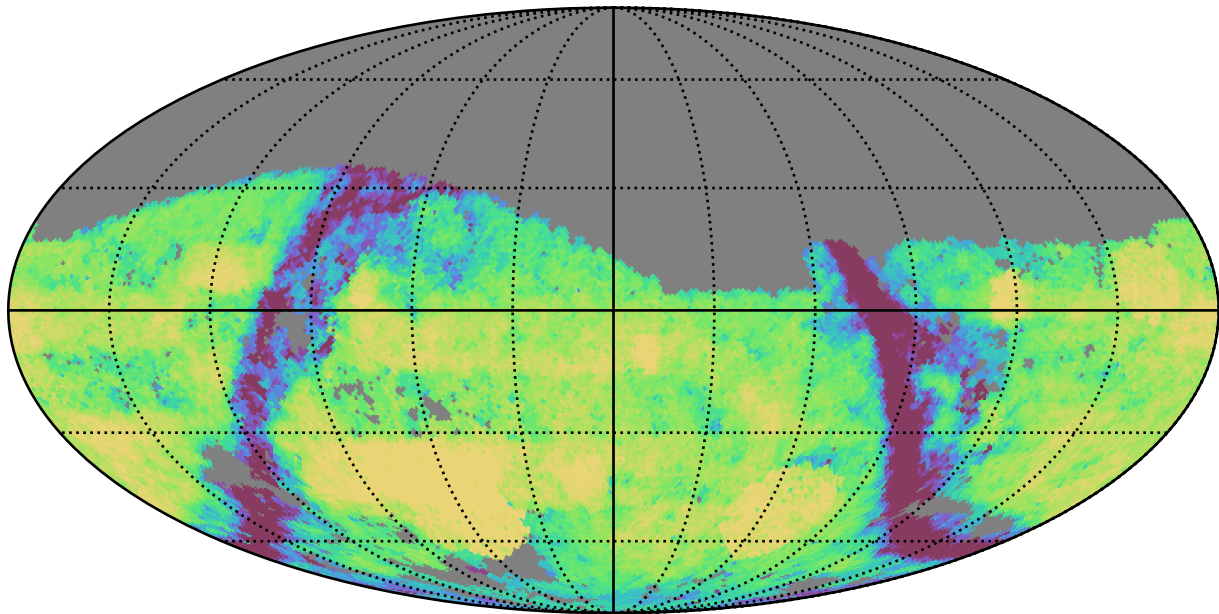
too_combined_s0.5_v3.4_10yrs Yr 3-4 g band: Exgal_CoaddM5
