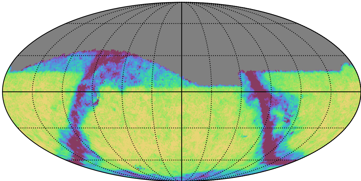
too_combined_s0.5_v3.4_10yrs Yr 1 z band: Exgal_CoaddM5
