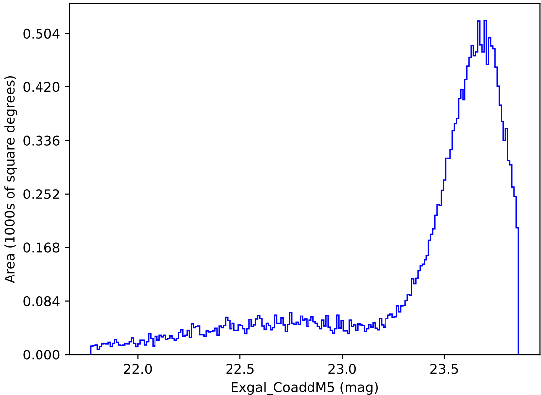
too_combined_s0.5_v3.4_10yrs Yr 1 y band: Exgal_CoaddM5
