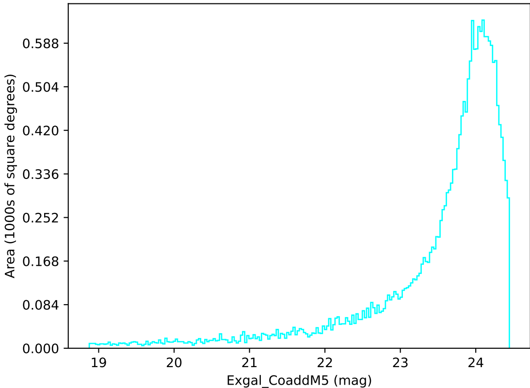
too_combined_s0.5_v3.4_10yrs Yr 1 u band: Exgal_CoaddM5
