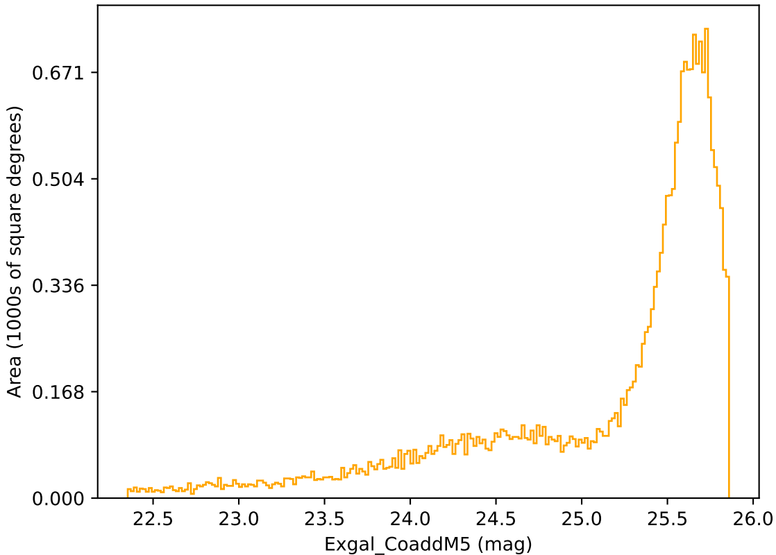
too_combined_s0.5_v3.4_10yrs Yr 1 r band: Exgal_CoaddM5
