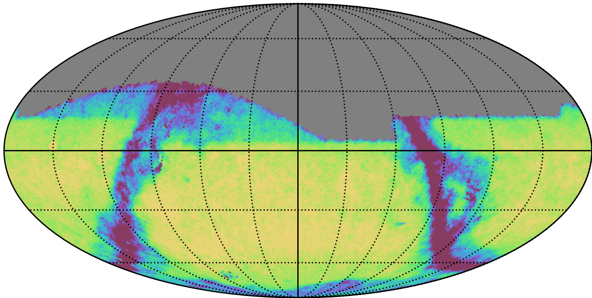
too_combined_s0.5_v3.4_10yrs Yr 1 i band: Exgal_CoaddM5
