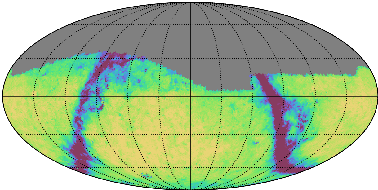
too_combined_s0.5_v3.4_10yrs Yr 1 g band: Exgal_CoaddM5
