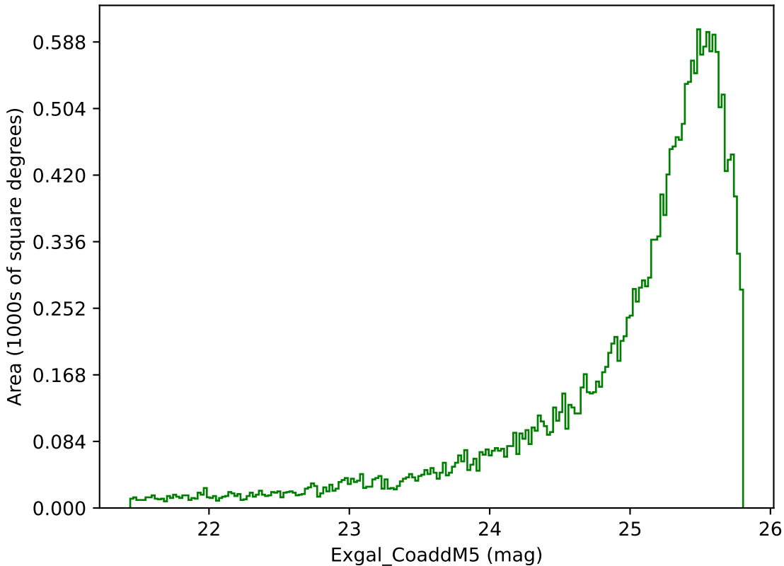
too_combined_s0.5_v3.4_10yrs Yr 1 g band: Exgal_CoaddM5
