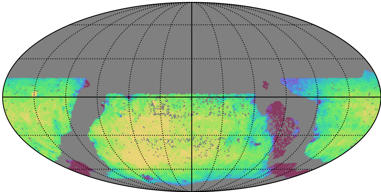
too_combined_s0.5_v3.4_10yrs WFD z band: Exgal_CoaddM5
