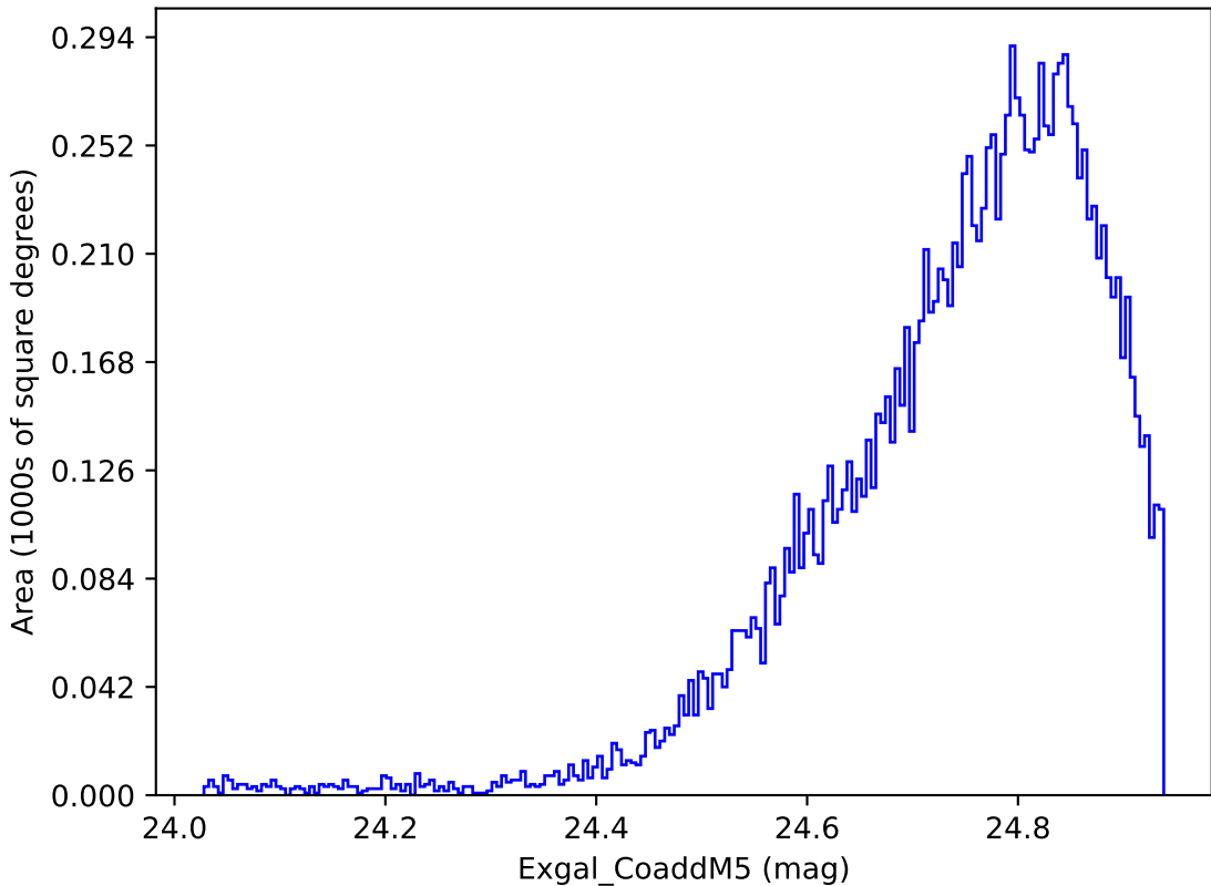
too_combined_s0.5_v3.4_10yrs WFD y band: Exgal_CoaddM5
