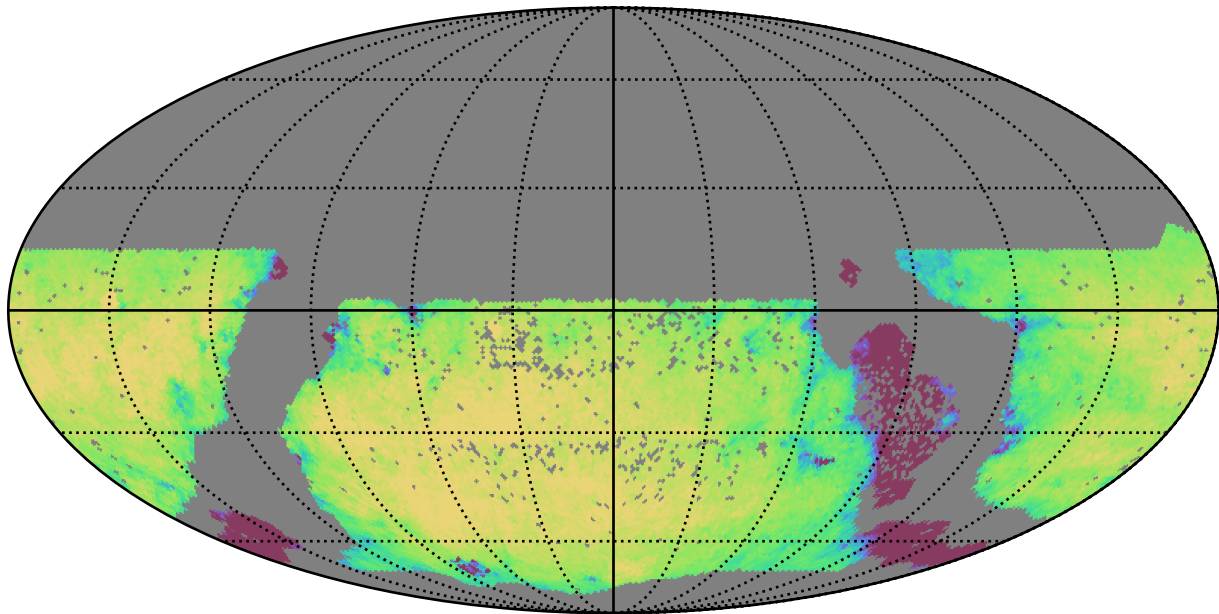
too_combined_s0.5_v3.4_10yrs WFD u band: Exgal_CoaddM5
