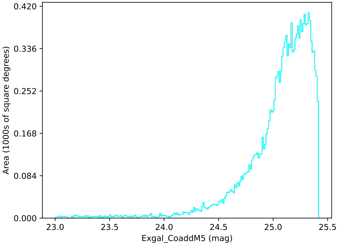
too_combined_s0.5_v3.4_10yrs WFD u band: Exgal_CoaddM5
