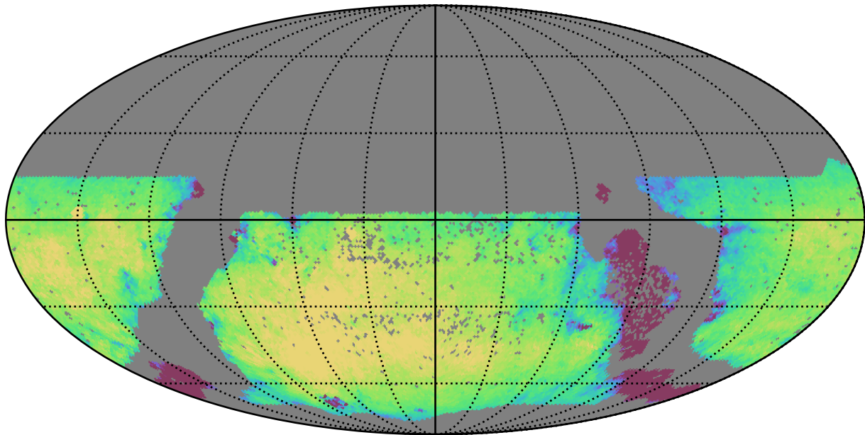
too_combined_s0.5_v3.4_10yrs WFD r band: Exgal_CoaddM5
