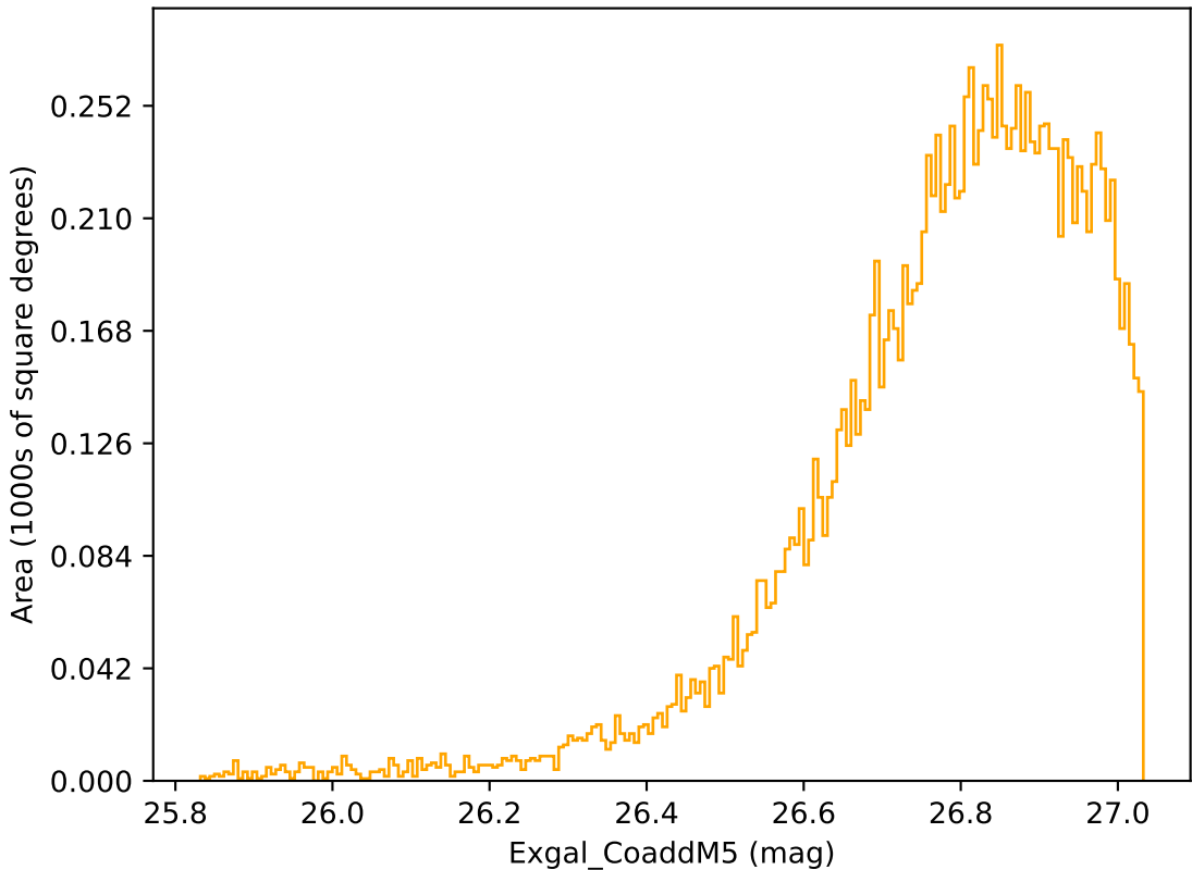
too_combined_s0.5_v3.4_10yrs WFD r band: Exgal_CoaddM5
