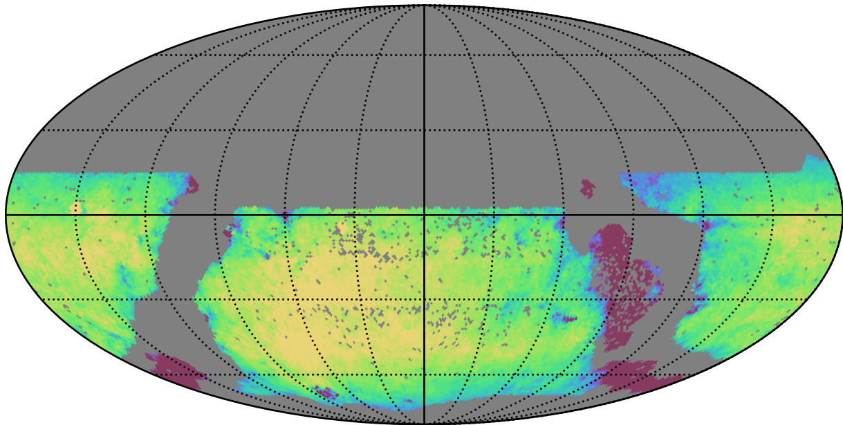
too_combined_s0.5_v3.4_10yrs WFD i band: Exgal_CoaddM5
