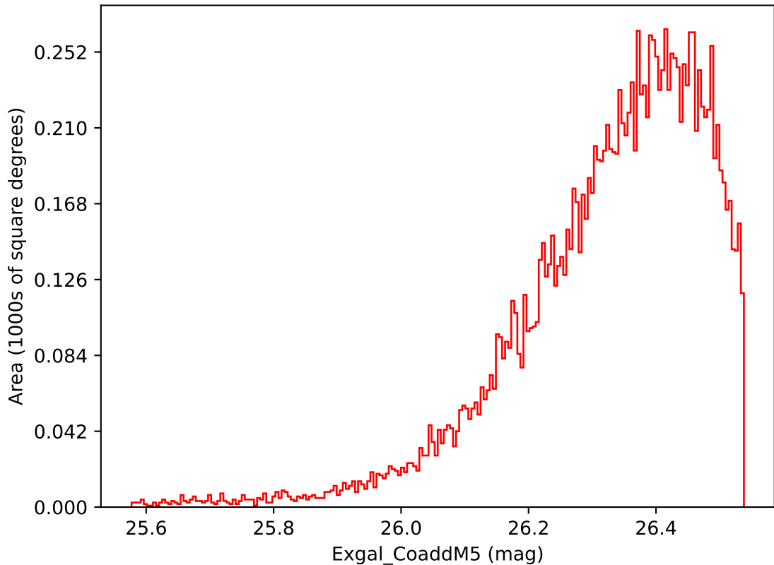
too_combined_s0.5_v3.4_10yrs WFD i band: Exgal_CoaddM5
