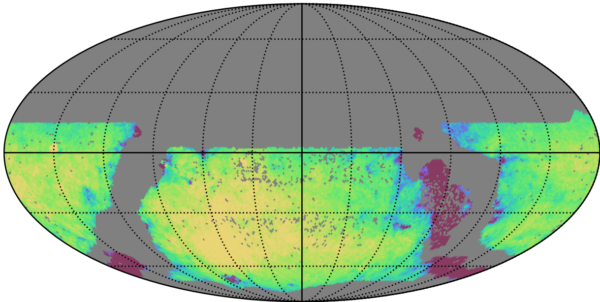
too_combined_s0.5_v3.4_10yrs WFD g band: Exgal_CoaddM5
