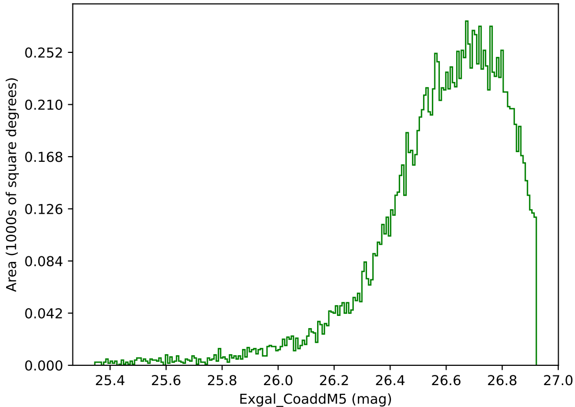
too_combined_s0.5_v3.4_10yrs WFD g band: Exgal_CoaddM5
