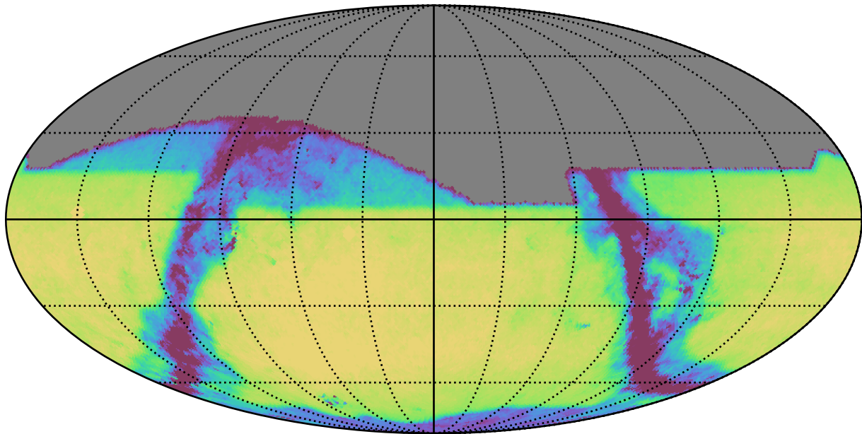
too_combined_s0.5_v3.4_10yrs All sky z band: Exgal_CoaddM5
