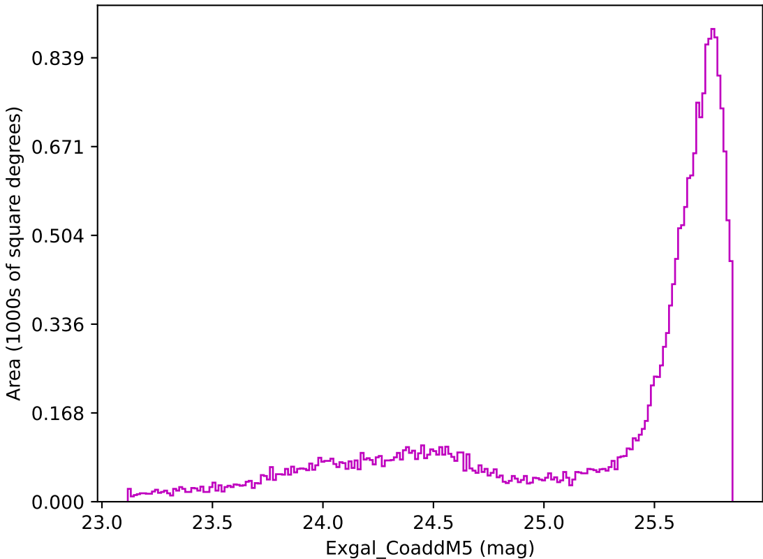
too_combined_s0.5_v3.4_10yrs All sky z band: Exgal_CoaddM5
