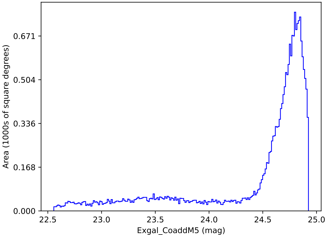
too_combined_s0.5_v3.4_10yrs All sky y band: Exgal_CoaddM5
