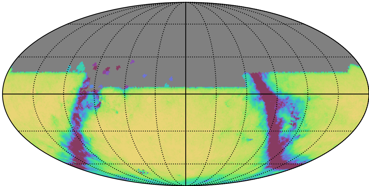
too_combined_s0.5_v3.4_10yrs All sky u band: Exgal_CoaddM5
