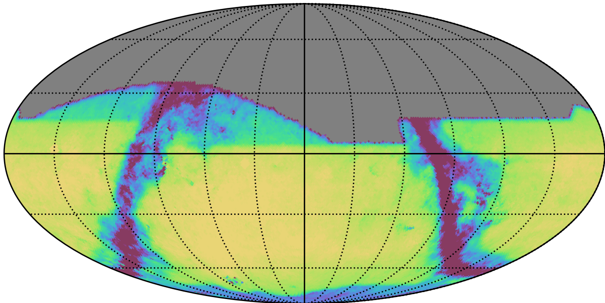
too_combined_s0.5_v3.4_10yrs All sky i band: Exgal_CoaddM5
