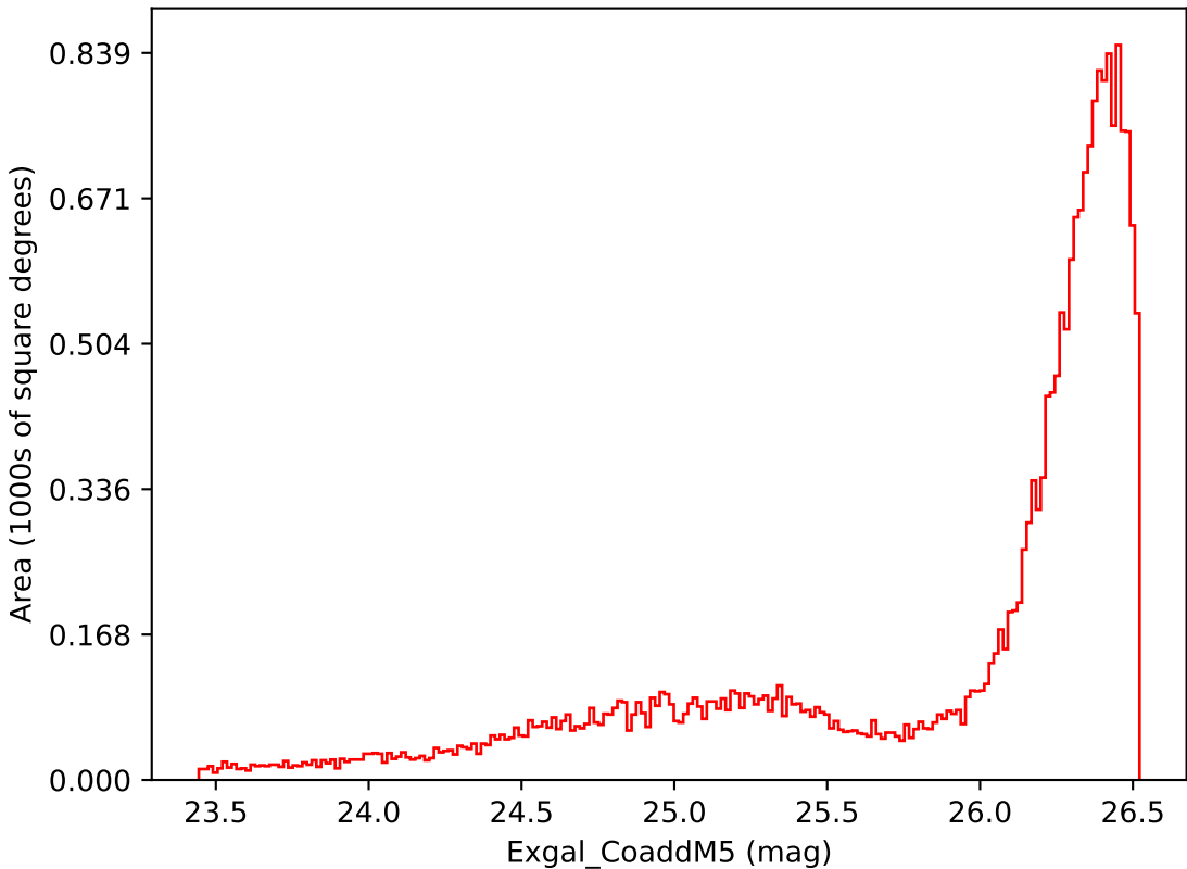
too_combined_s0.5_v3.4_10yrs All sky i band: Exgal_CoaddM5
