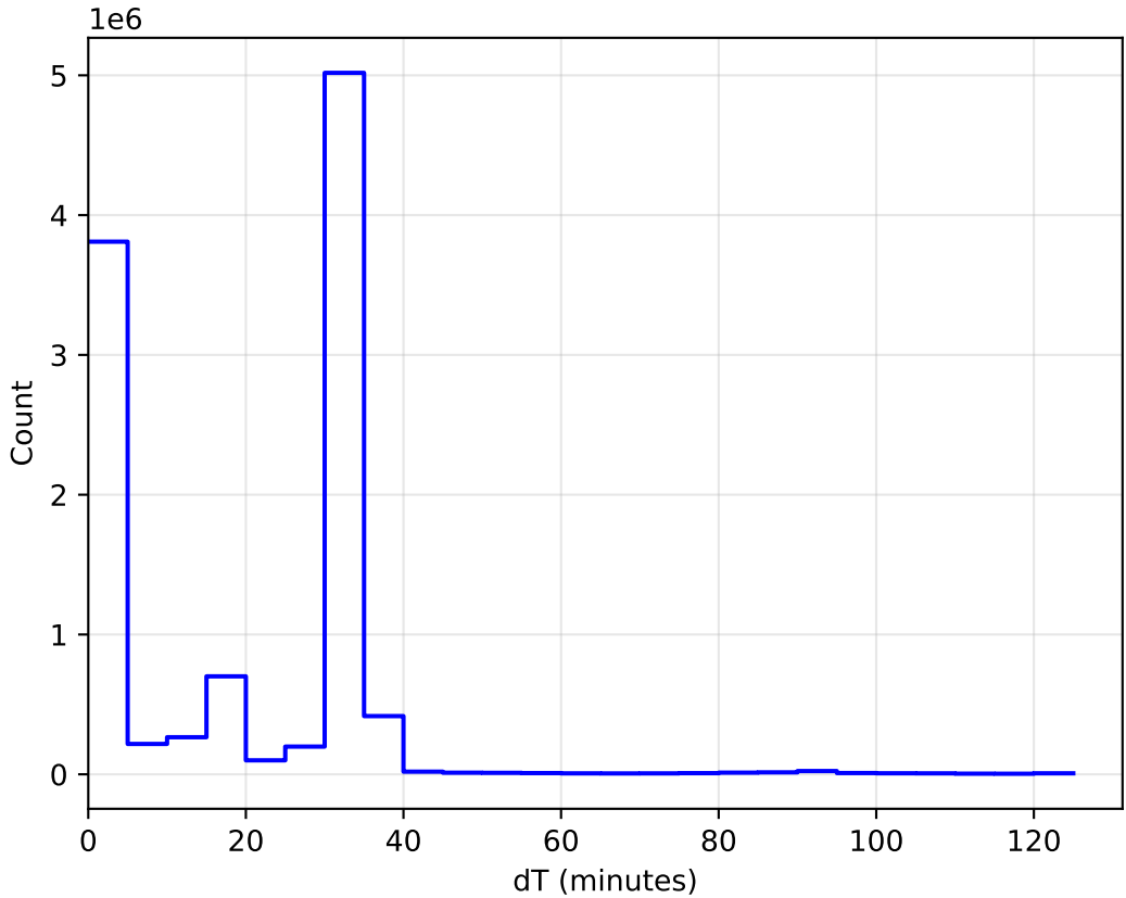
too_combined_s0.5_v3.4_10yrs WFD: DeltaT Histogram
