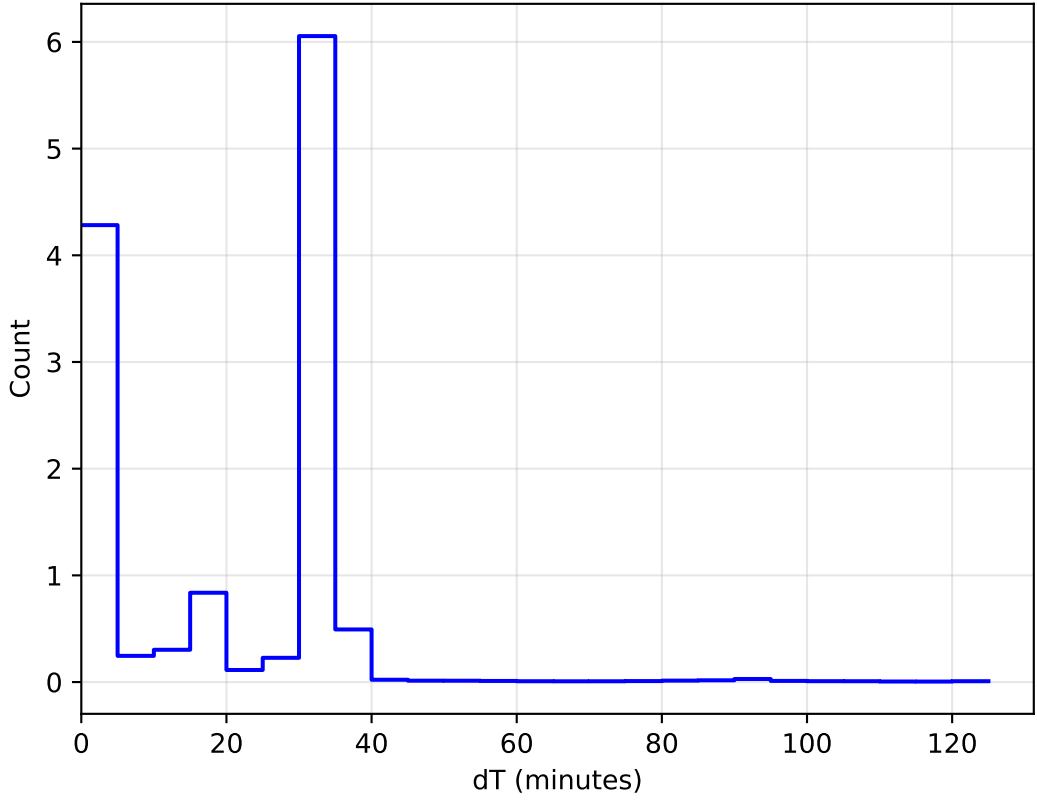
too_combined_s0.5_v3.4_10yrs All sky: DeltaT Histogram
