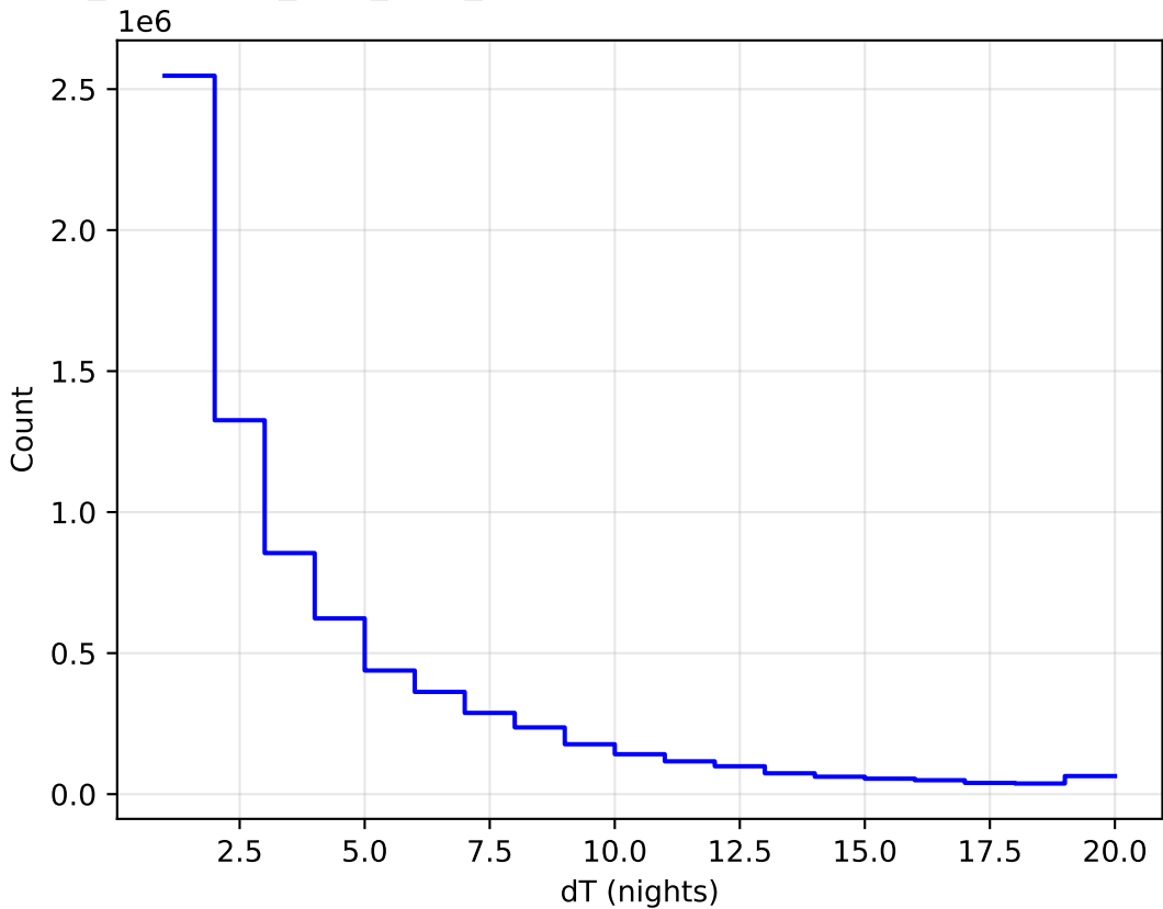
too_combined_s0.5_v3.4_10yrs WFD all bands: DeltaNight Histogram
