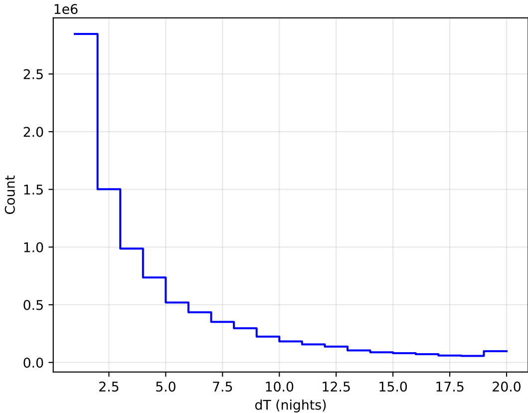
too_combined_s0.5_v3.4_10yrs All sky all bands: DeltaNight Histogram
