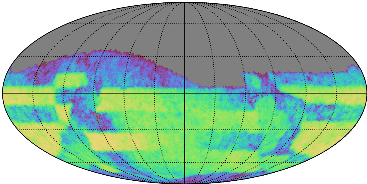
too_combined_s0.5_v3.4_10yrs Yr 3-4 z band: CoaddM5
