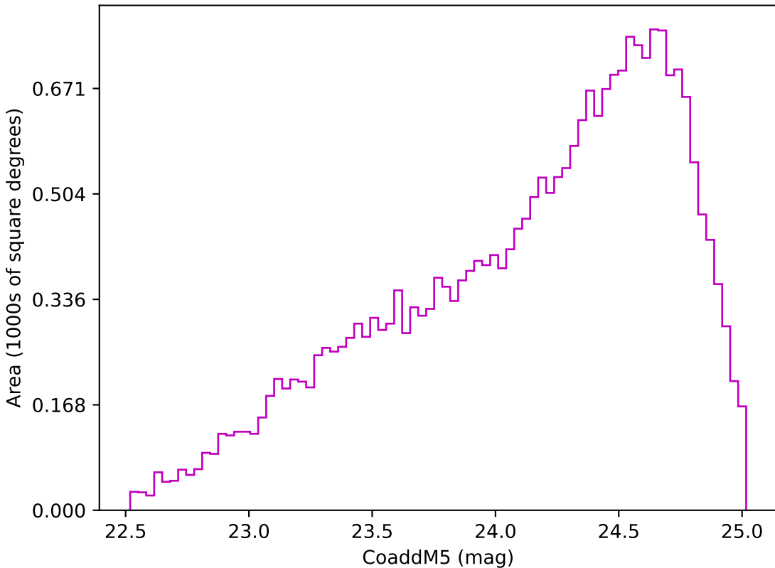
too_combined_s0.5_v3.4_10yrs Yr 3-4 z band: CoaddM5
