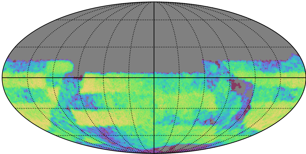
too_combined_s0.5_v3.4_10yrs Yr 3-4 y band: CoaddM5
