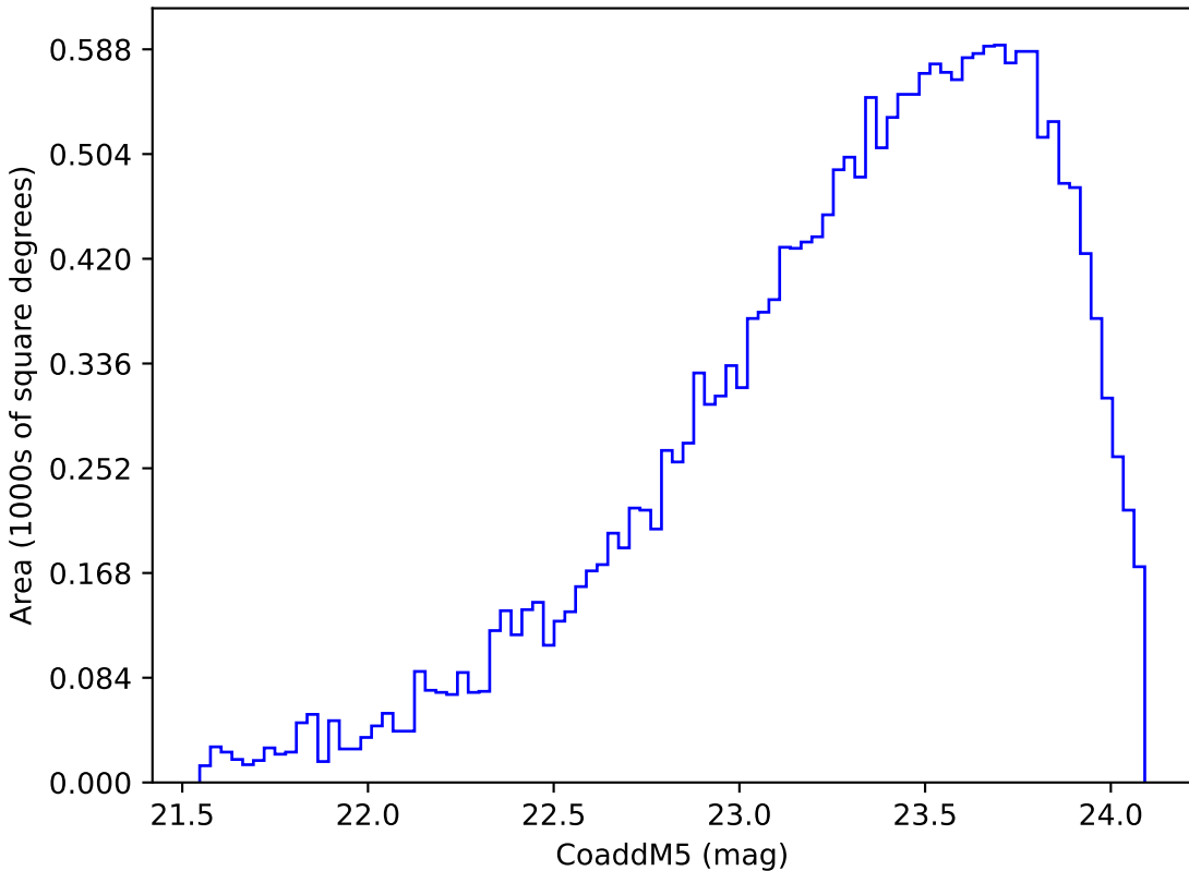
too_combined_s0.5_v3.4_10yrs Yr 3-4 y band: CoaddM5
