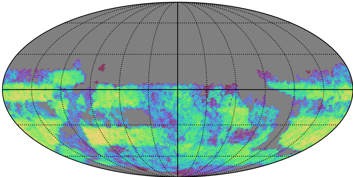
too_combined_s0.5_v3.4_10yrs Yr 3-4 u band: CoaddM5
