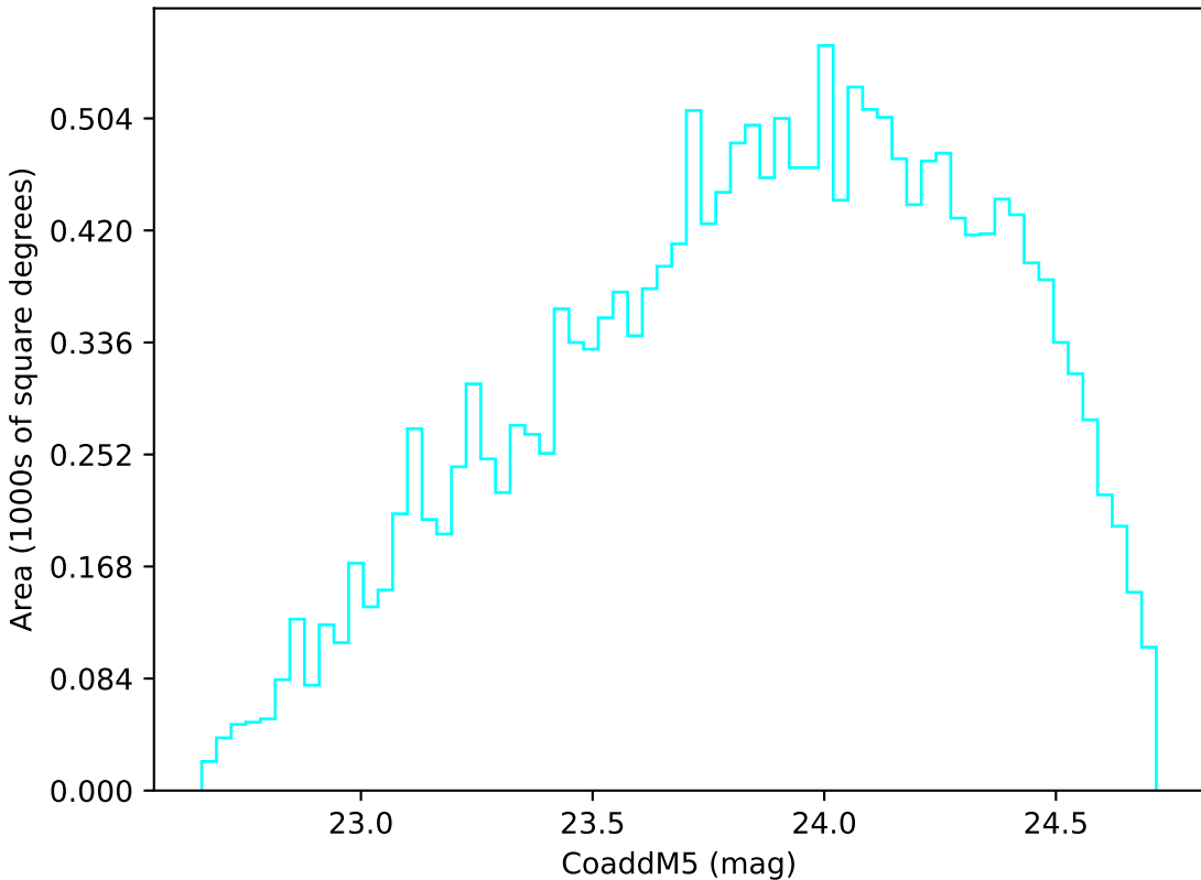
too_combined_s0.5_v3.4_10yrs Yr 3-4 u band: CoaddM5
