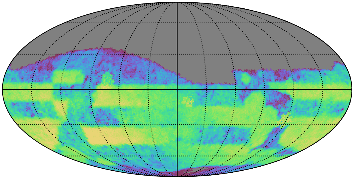
too_combined_s0.5_v3.4_10yrs Yr 3-4 r band: CoaddM5
