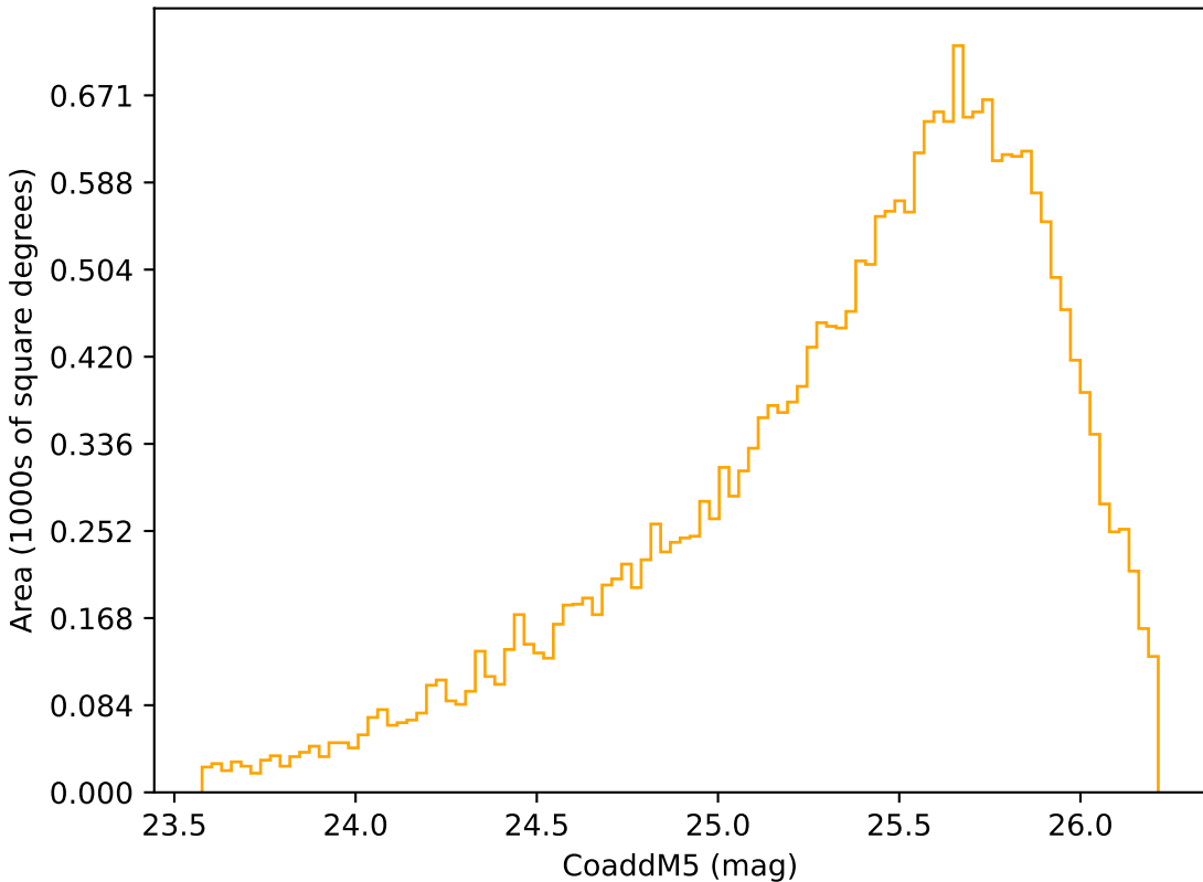
too_combined_s0.5_v3.4_10yrs Yr 3-4 r band: CoaddM5
