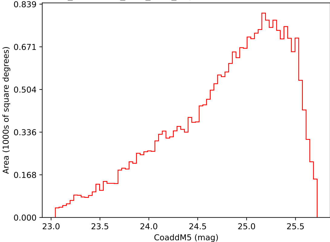
too_combined_s0.5_v3.4_10yrs Yr 3-4 i band: CoaddM5
